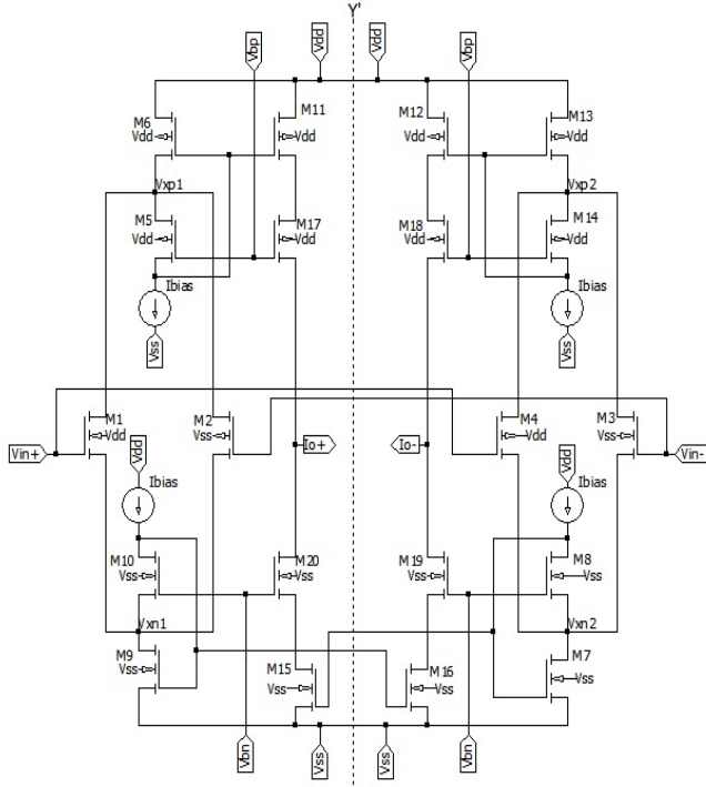
Fig. 3: OTA circuit
