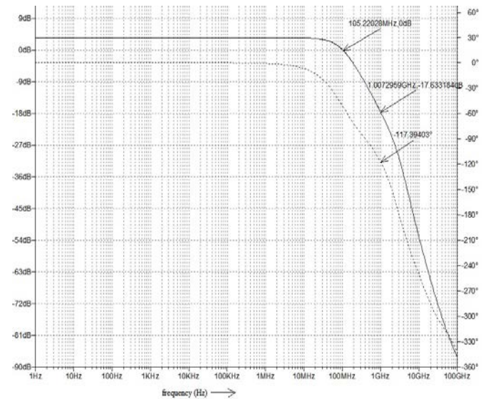
Fig. 51: Frequency response of the transconductor.
