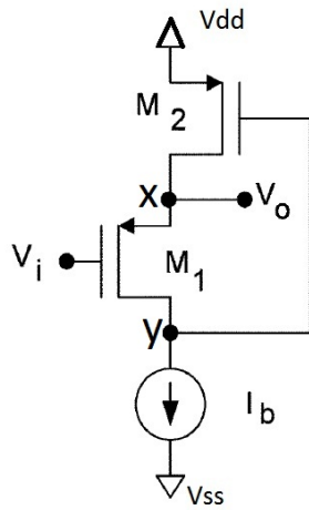
Fig. 1: Flipped voltage follower
